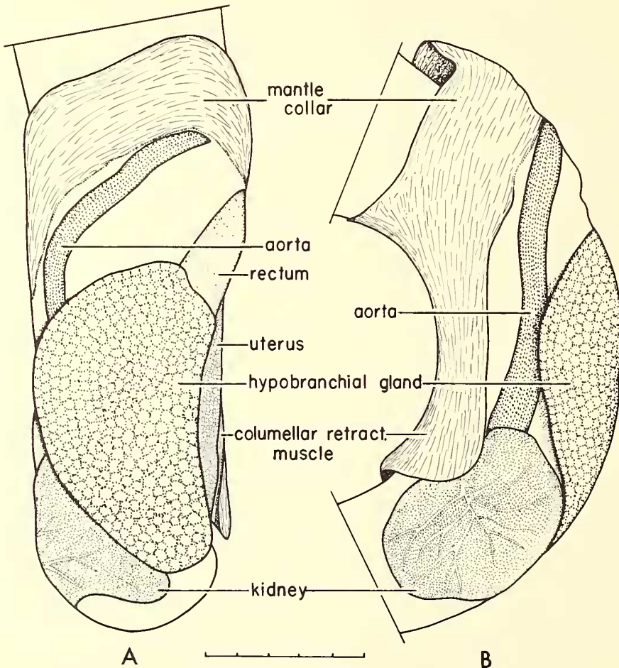
TEXT-FIG. 1. Aperostoma palmeri (Bartsch and Morrison). Dorsal and lateral view of the pseudolung and associated organs showing the relatively large hypobranchial gland. Scale equals 5 mm.
